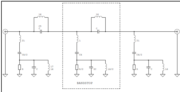
Figure 13 – Hagerman Absorptive Band Stop Filter Schematic
