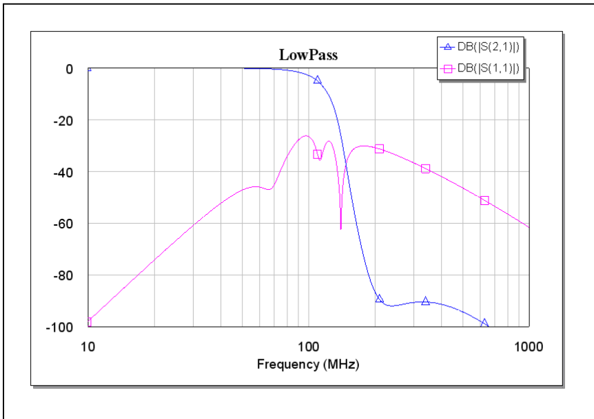
Figure 6 – Simulation Results of Figure 4
