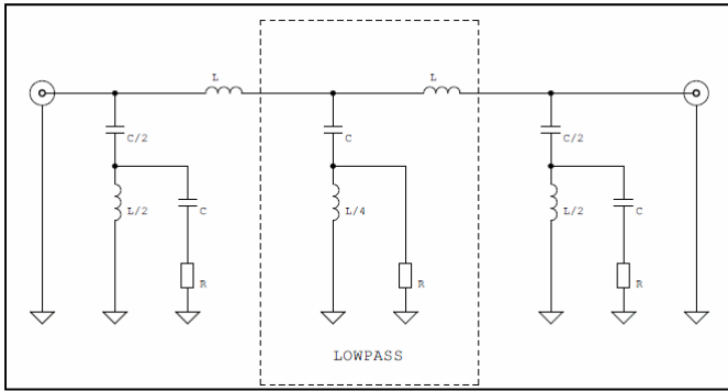
Figure 4 – Hagerman Absorptive Low Pass Filter Schematic
