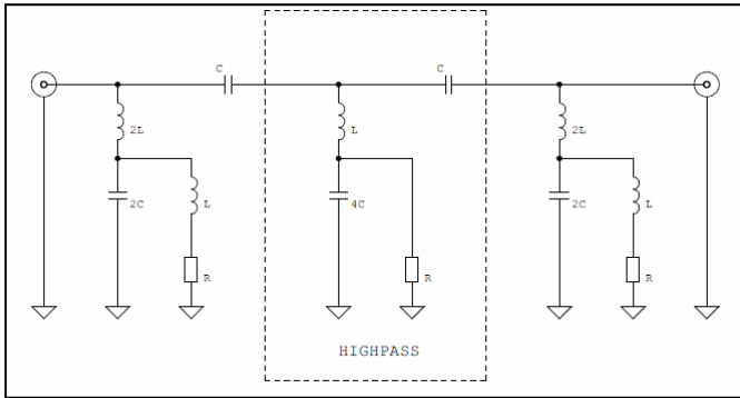
Figure 7 – Hagerman Absorptive High Pass Filter Schematic
