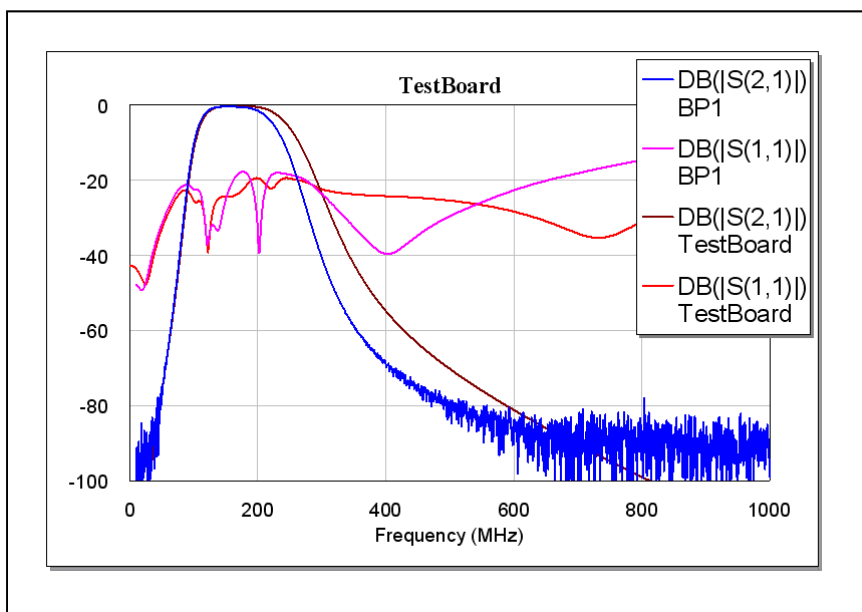
Figure 22 – Measured Results of Figure 21
