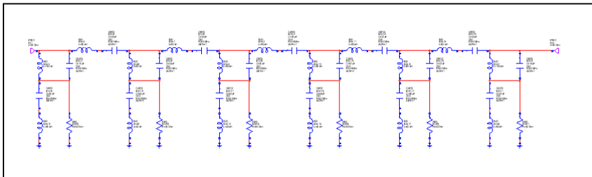
Figure 11 – Five Section Hagerman Absorptive Band Pass
