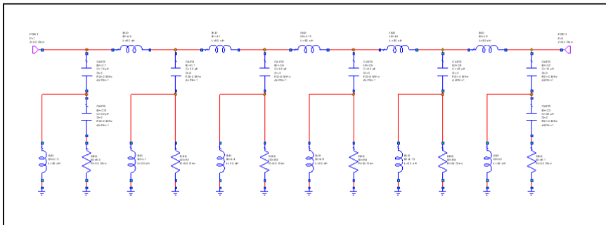
Figure 5 – Five Section Hagerman Absorptive Low Pass
