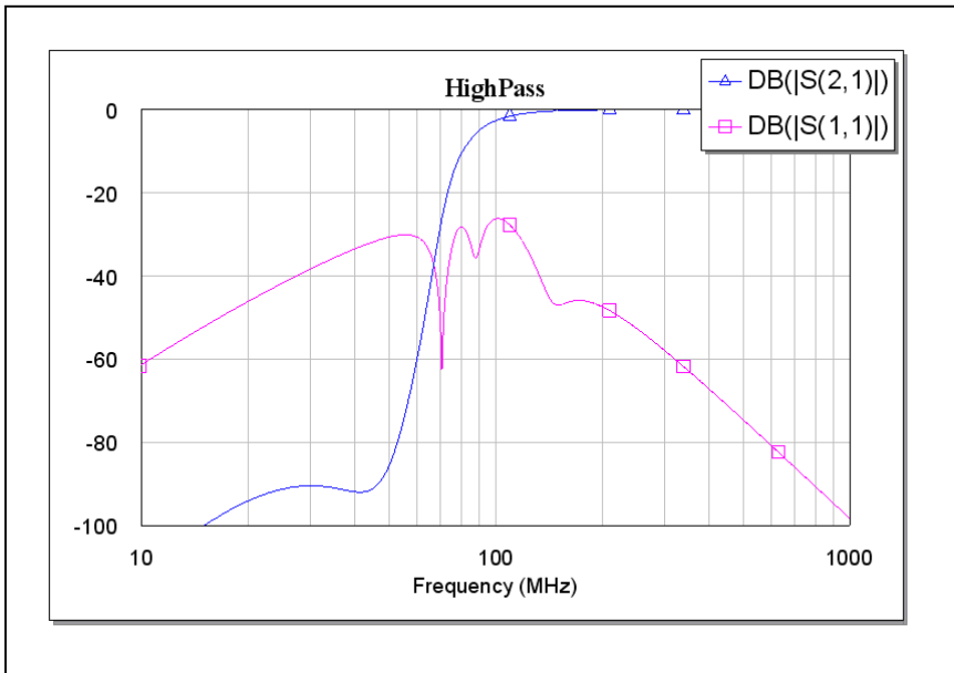
Figure 9 – Simulation Results of Figure 7
