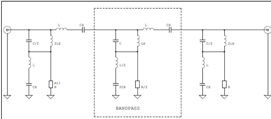
Figure 10 – Hagerman Absorptive Band Pass Filter Schematic
