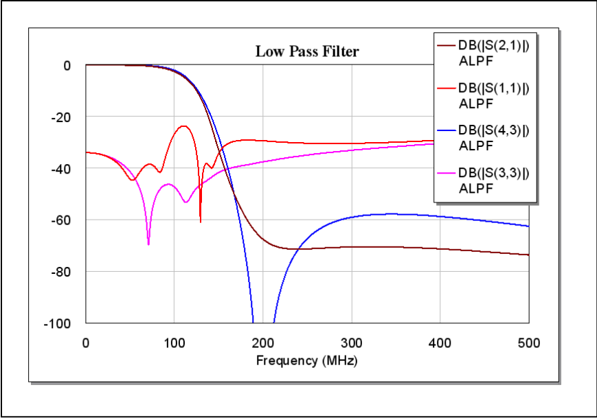
Figure 18 – Comparison of Morgan and Hagerman Low Pass Filters, Practical
