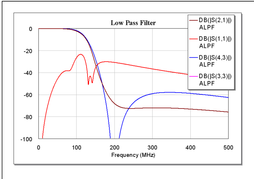
Figure 16 – Comparison of Morgan and Hagerman Low Pass Filters, Ideal
