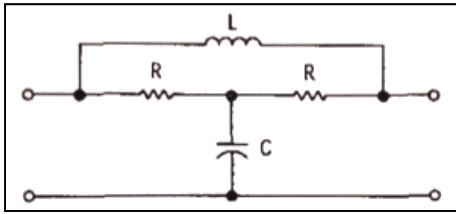
Figure 1 – Cuthbert Invulnerable Filter Schematic
