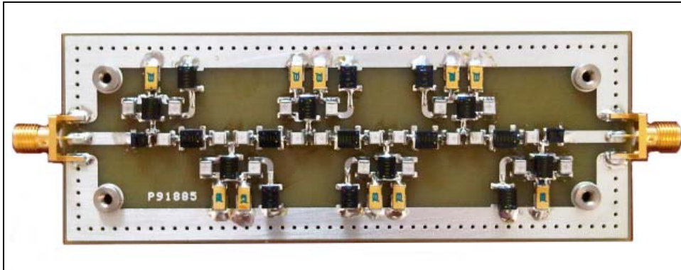
Figure 21 – Photo of Hagerman Absorptive Band Pass Breadboard
