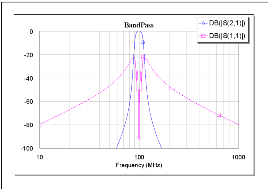
Figure 12 – Simulation Results of Figure 10
