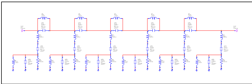
Figure 14 – Five Section Hagerman Absorptive Band Stop
