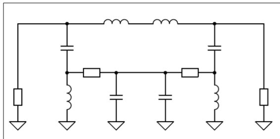
Figure 2 – Morgan Reflectionless Low Pass Filter Schematic
