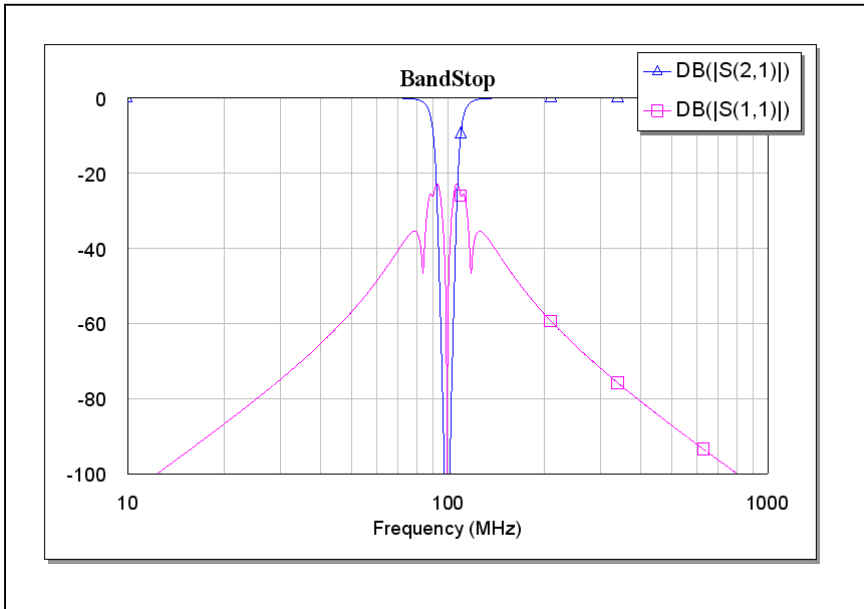
Figure 15 – Simulation Results of Figure 13
