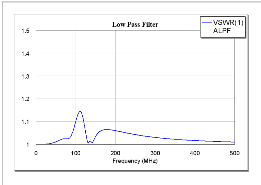
Figure 17 – VSWR of Hagerman Low Pass
