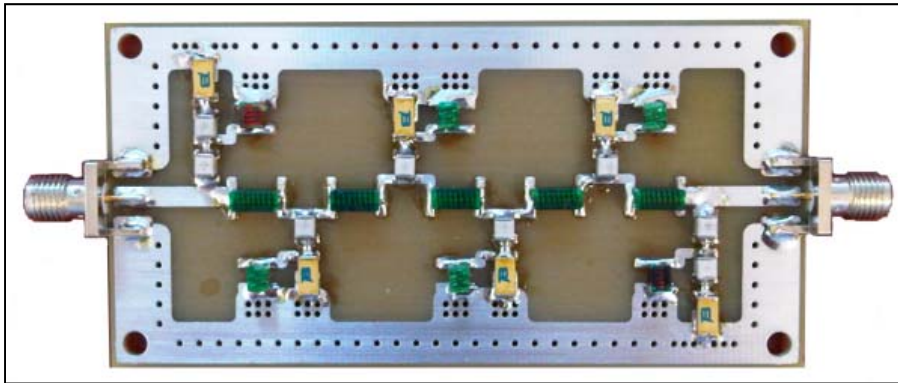
Figure 19 – Photo of Hagerman Absorptive Low Pass Breadboard
