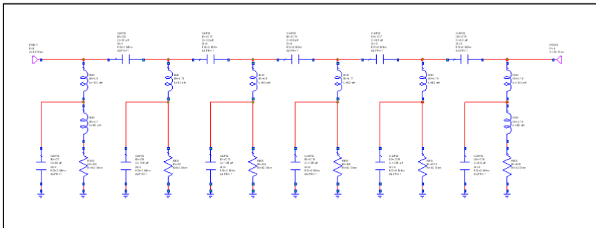
Figure 8 – Five Section Hagerman Absorptive High Pass
