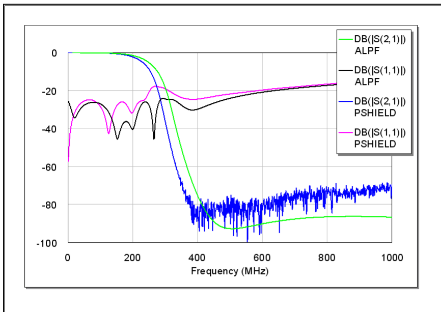
Figure 20 – Measured Results of Figure 19
